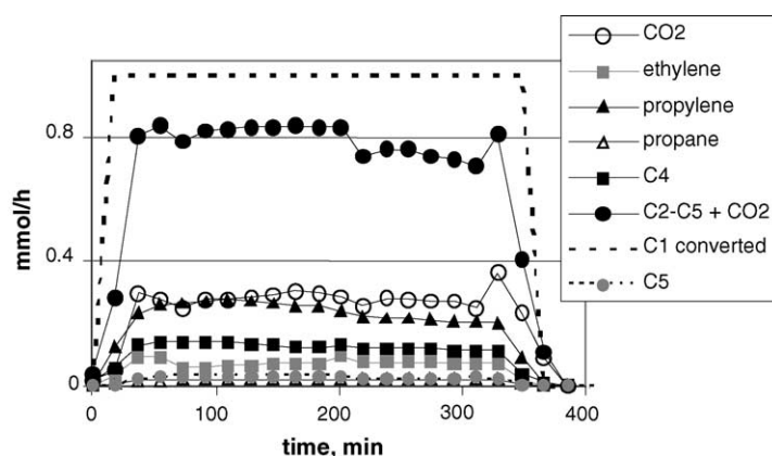
Fig. 4. Reactions products from a reactor into which \text{O}_2 is flowed at 0.3 \text{ cm}^3/\text{min} into a metal bromide bed, releasing bromine. The internally formed bromine is then mixed with methane ( 5 \text{ cm}^3/\text{min} ) and reacted at 415^\circ\text{C} to effect methane bromination. The methane bromination products are then passed over a complementary \text{CaO/ZSM-5} bed for coupling and bromine sequestration. The bromine moves through the reactor but never leaves the apparatus. The product distribution is nearly identical to that seen in Fig. 1.
