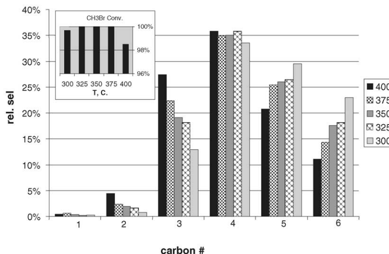
Fig. 2. \text{CH}_3\text{Br} (13 mmol) coupling products over Ca/ZSM-5 (5 g) as a function of temperature in ^\circ\text{C} . Conditions: P(\text{CH}_3\text{Br}) = 1 bar, WHSV = 2\text{ h}^{-1} , feed bed residence time \sim 3 s. \text{CH}_3\text{Br} reaction at each temperature was followed by regeneration of the bed with \text{O}_2 to recover \text{Br}_2 . Carbon # = 2 represents ethene, 3 represents propene, 4 represents a mixture of butenes, with trace butanes, 5 and 6 represent all pentenes and pentanes and hexenes and hexanes, respectively. Inset shows methyl bromide conversion.
